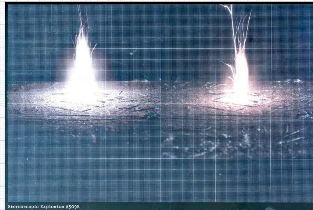
Stereoscopic Explosion #5098
