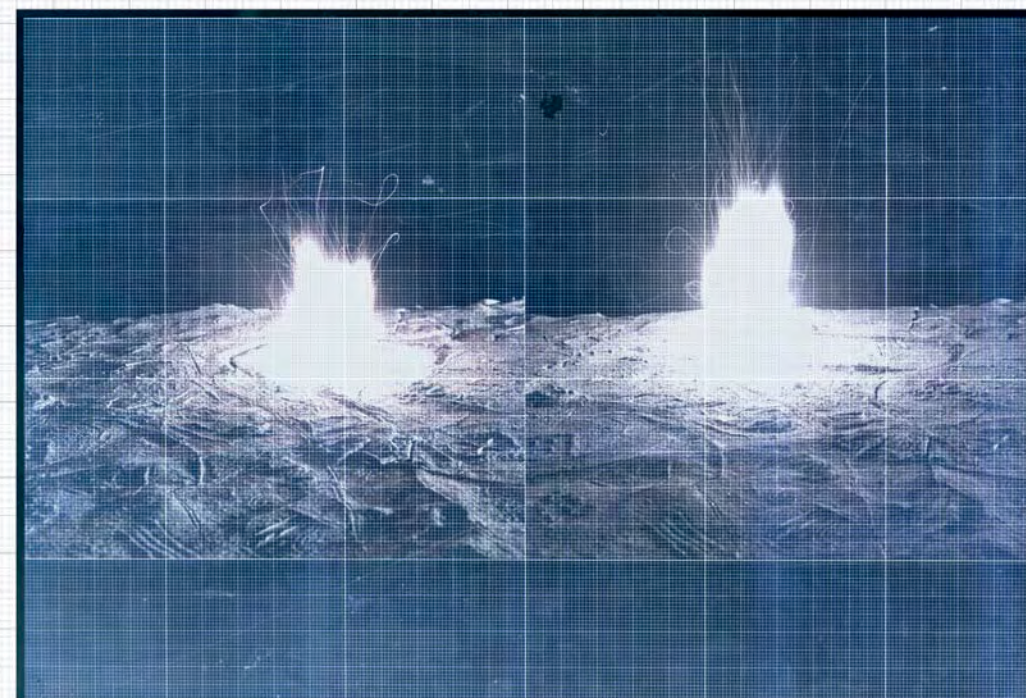
Stereoscopic Explosion #5099
